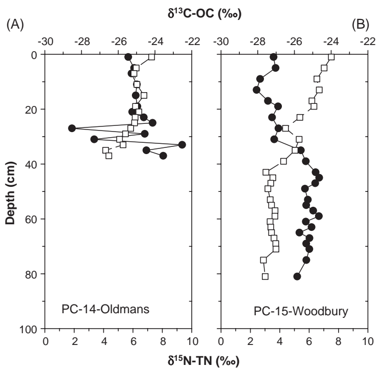
Fig. 5. Carbon (●) and nitrogen (□) isotopic composition with depth in (A) Oldmans and (B) Woodbury Creek marshes from the upper Delaware estuary.
