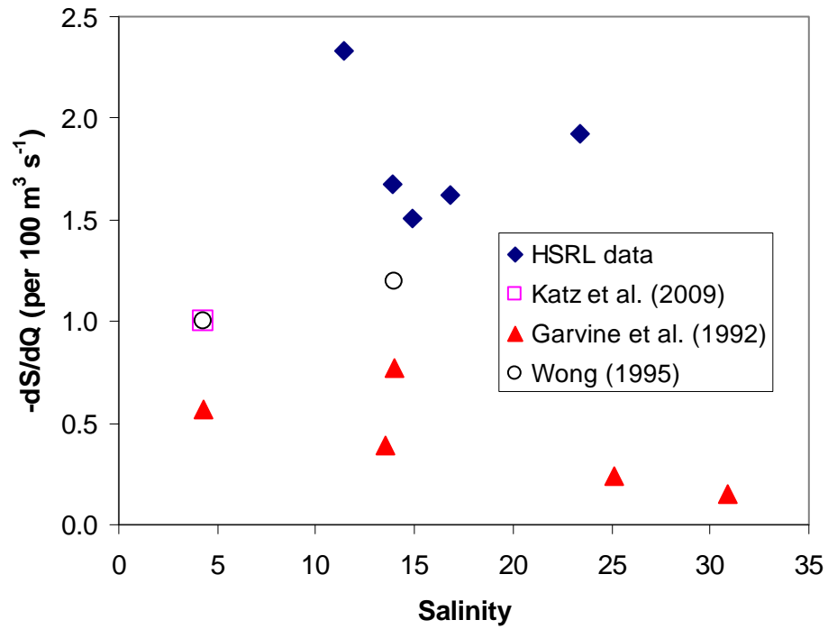
Fig. 5. Summary of estimates of the sensitivity of Delaware Estuary salinity ( S ) to streamflow at Trenton ( Q ) as a function of salinity. HSRL = Haskin Shellfish Research Laboratory.
