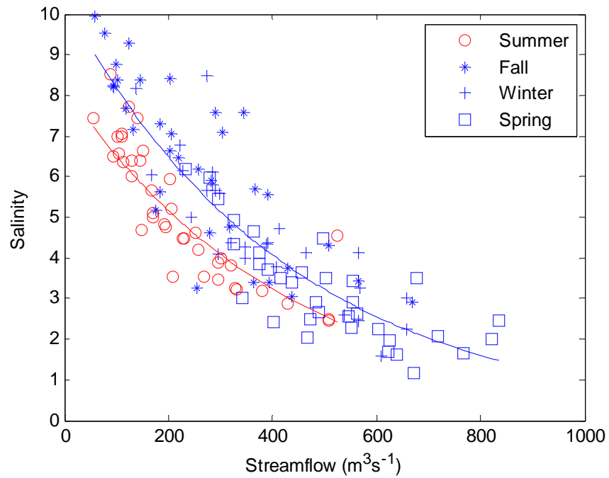
Fig. 4. Monthly mean salinity at Reedy Island Jetty as a function of monthly mean Trenton streamflow (not lagged). The symbols represent individual seasons and the lines are least-squares exponential fits to summer data (red) and data from the other seasons combined (blue). From Katz et al. (2010).
