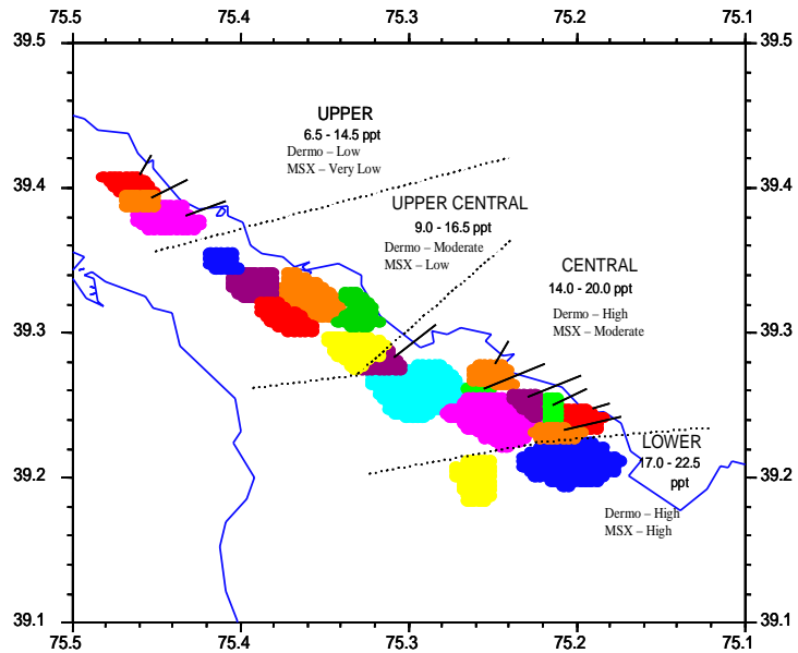
Figure N-5. New Jersey seed beds of Crassostrea virginica in relation to salinity and disease susceptibility.
