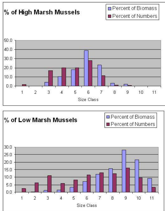
Figure N-3. Average densities and sizes (cm shell height) of ribbed mussels living in tidal marshes fringing the Broadkill River of lower Delaware (Kreeger unpublished.)
