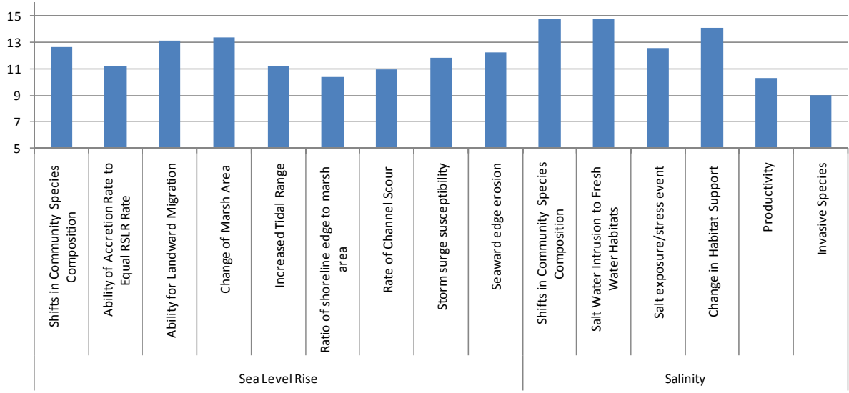
Figure H.1.4 Freshwater Tidal Wetland – Combined Impacts and Confidence for Vulnerabilities to Sea Level Rise and Salinity
