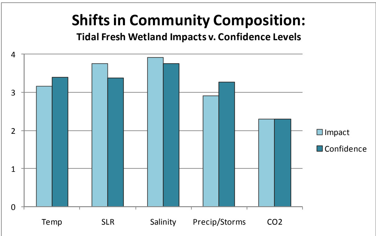
Figure H.1.1 Freshwater Tidal Wetland – Impacts v. Confidence of Species Composition Shifts
