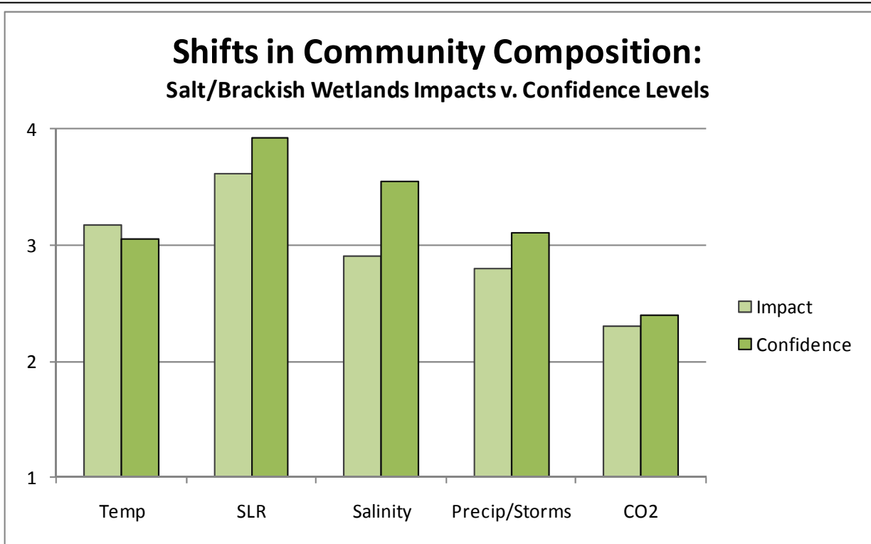
Figure H.1.2 Salt/Brackish Tidal Wetland – Impacts v. Confidence of Species Composition Shifts
