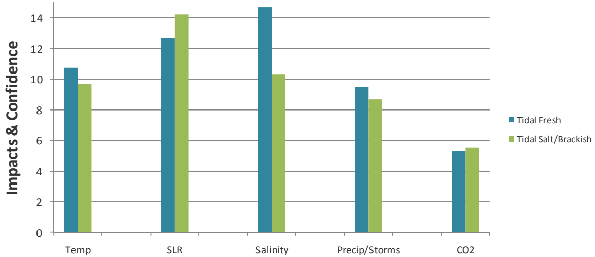
Figure H.1.3 Freshwater & Salt/Brackish Tidal Wetland – Combined Impacts and Confidence for Species Composition Shifts
